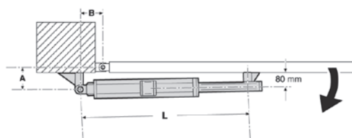
Operators wit 265 mm piston rod For 90° opening angle (mm) A max: 175 mm B min. (90°): 80 mm L: 985 mm
