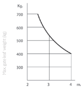
Max. gate leaf length (m) Operators wit 265 mm piston rod
